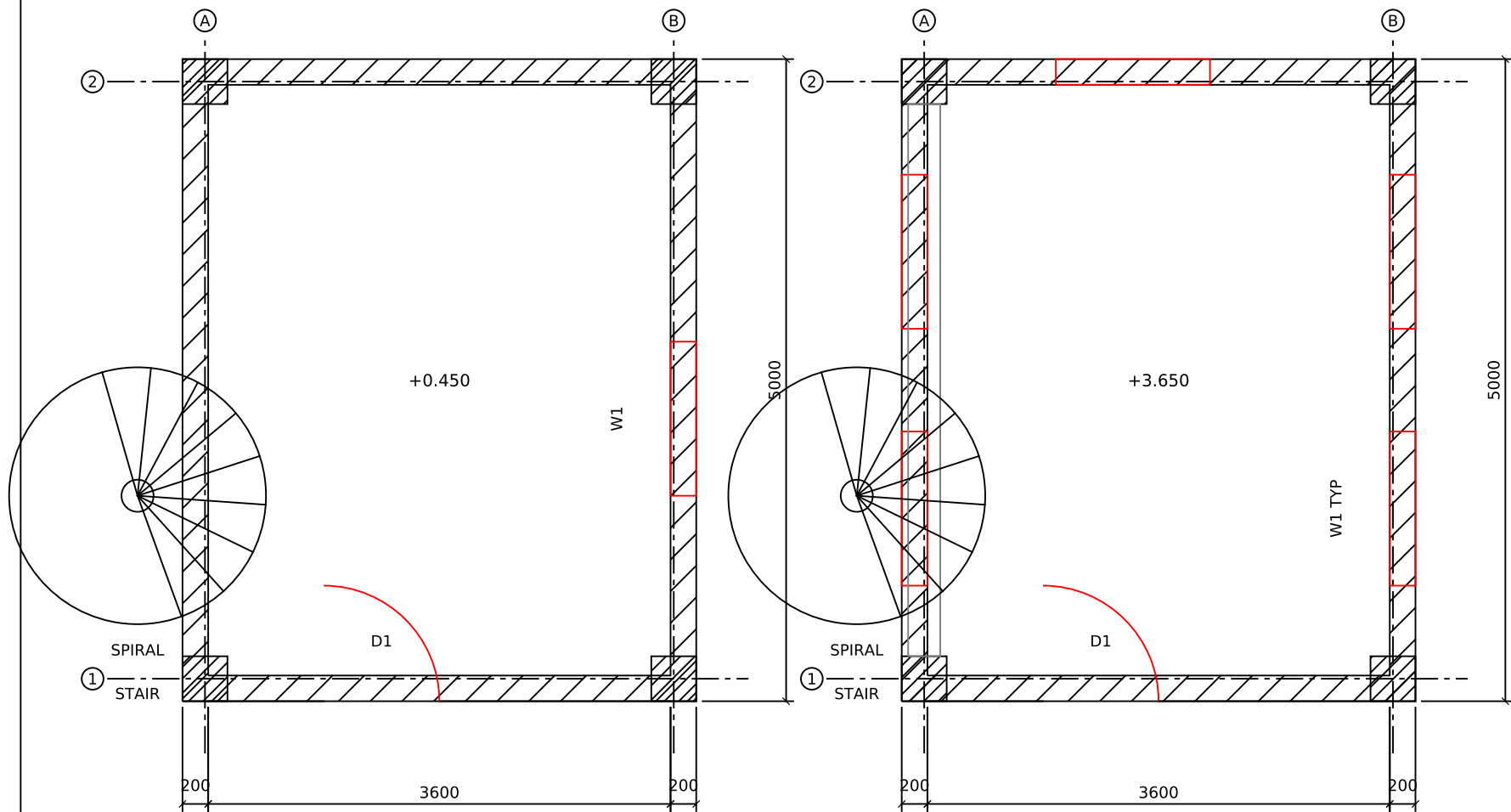
1 GROUND FLOOR LEVEL 1 : 50 FFL +0.450
