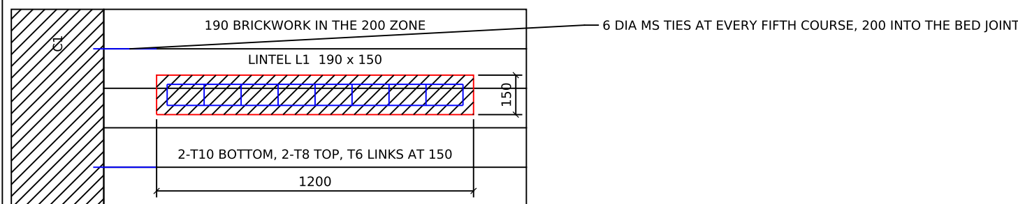
4 LINTEL L1, WALL TIES AND THE 200 INFILL ZONE 1 : 20 ONE LINTEL TYPE SERVES ALL ELEVEN OPENINGS
