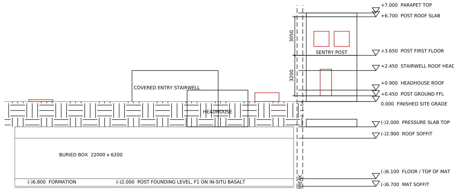
3 SOUTH ELEVATION - SHELTER AND SENTRY POST 1 : 150 SENTRY POST AT TRUE X ACROSS A BREAK
